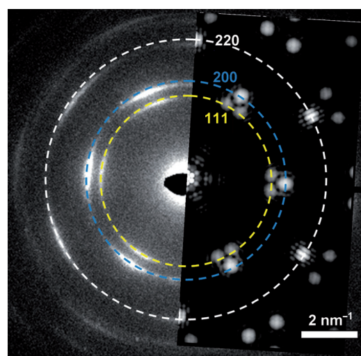
Figure 6. Comparison of the observed (left) and simulated (right) ED patterns detected along [111]_{SL} of the PbS–organic mesocrystal. The simulated ED was obtained by superposition of the ED patterns calculated for the proposed models II and III (see Figure 5). The sets of equidistant (220) , (002) , and (111) PbS Bragg reflections are marked with white, blue, and yellow circles, respectively.
