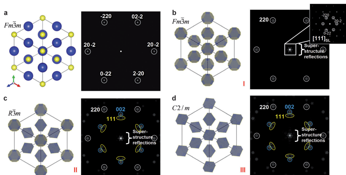
Figure 5. a) [111] Projection of the galena (PbS) crystal structure with corresponding simulated SAED pattern. [111]_{SL} Projections of simulated PbS–organic colloidal crystals (models I (b), II (c), and III (d)) with corresponding simulated ED patterns, illustrating orientational relationships between the superstructure and the PbS (galena) nanocrystal reflections. The sets of equidistant (220) , (002) , and (111) PbS Bragg reflections are marked with white, blue, and yellow circles, respectively. In model I (b), truncated octahedrally shaped PbS nanoparticles are placed at the nodes of the fcc superlattice where the [111]_{PbS} orientations of the nanoparticles are parallel with the [111]_{SL} superlattice orientation. In model II (c), along [111]_{SL} of superlattice, nanoparticles at the centers of fcc unit-cell faces have a [110]_{PbS} orientation, while at the vertices [111]_{PbS} . Finally, in model III (d), all nanoparticles show the [110]_{PbS} orientation parallel to the [111]_{SL} zone of the superlattice. Nanoparticle habits and orientations are taken from Figure 3.
